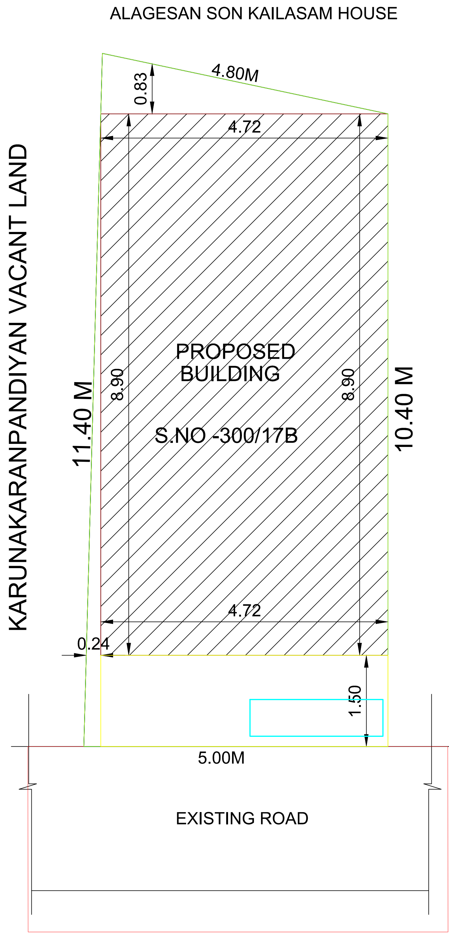
SITE PLAN
