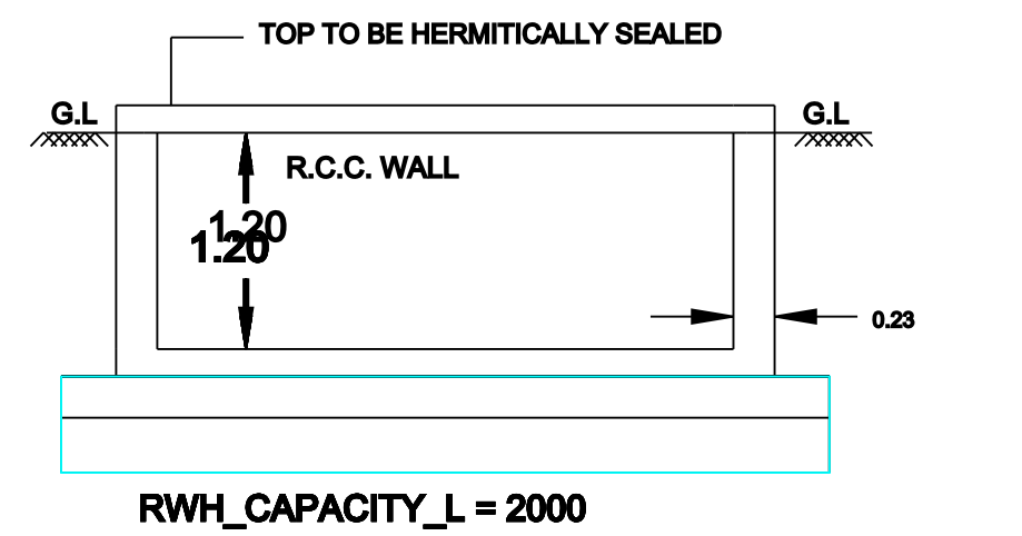
RAIN WATER HARVESTING ARRANGEMENT
