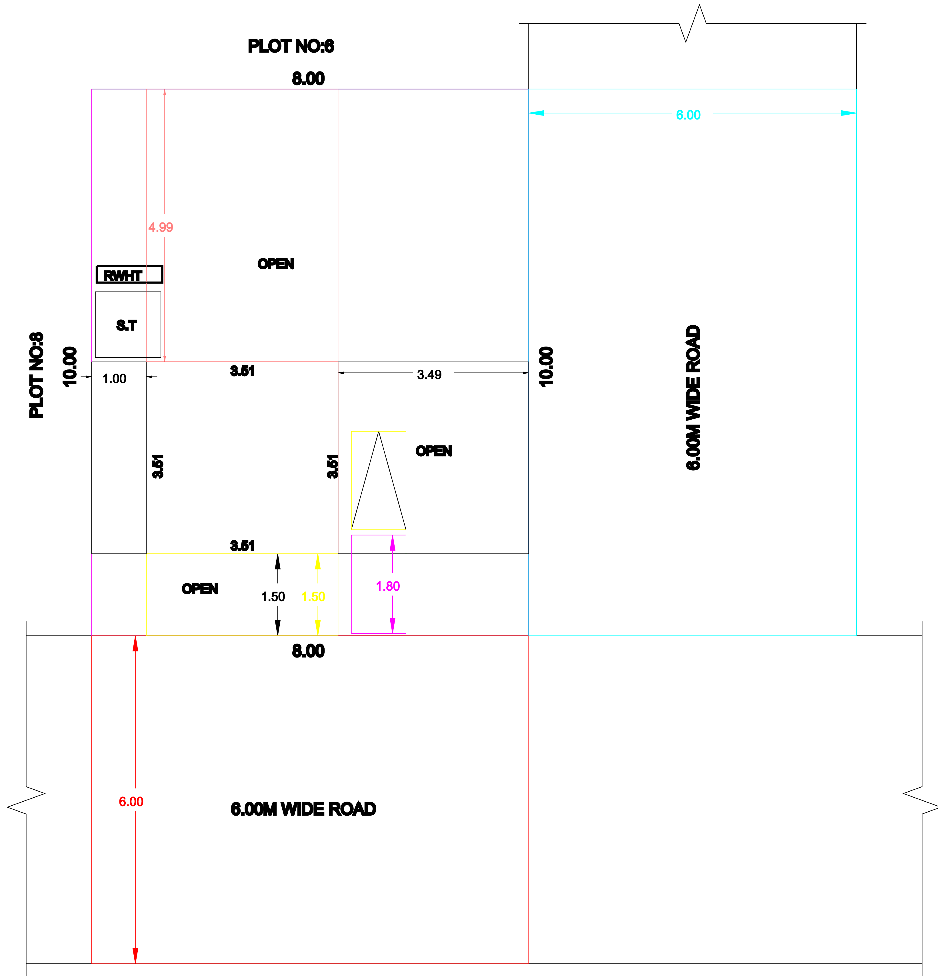
SITE PLAN
