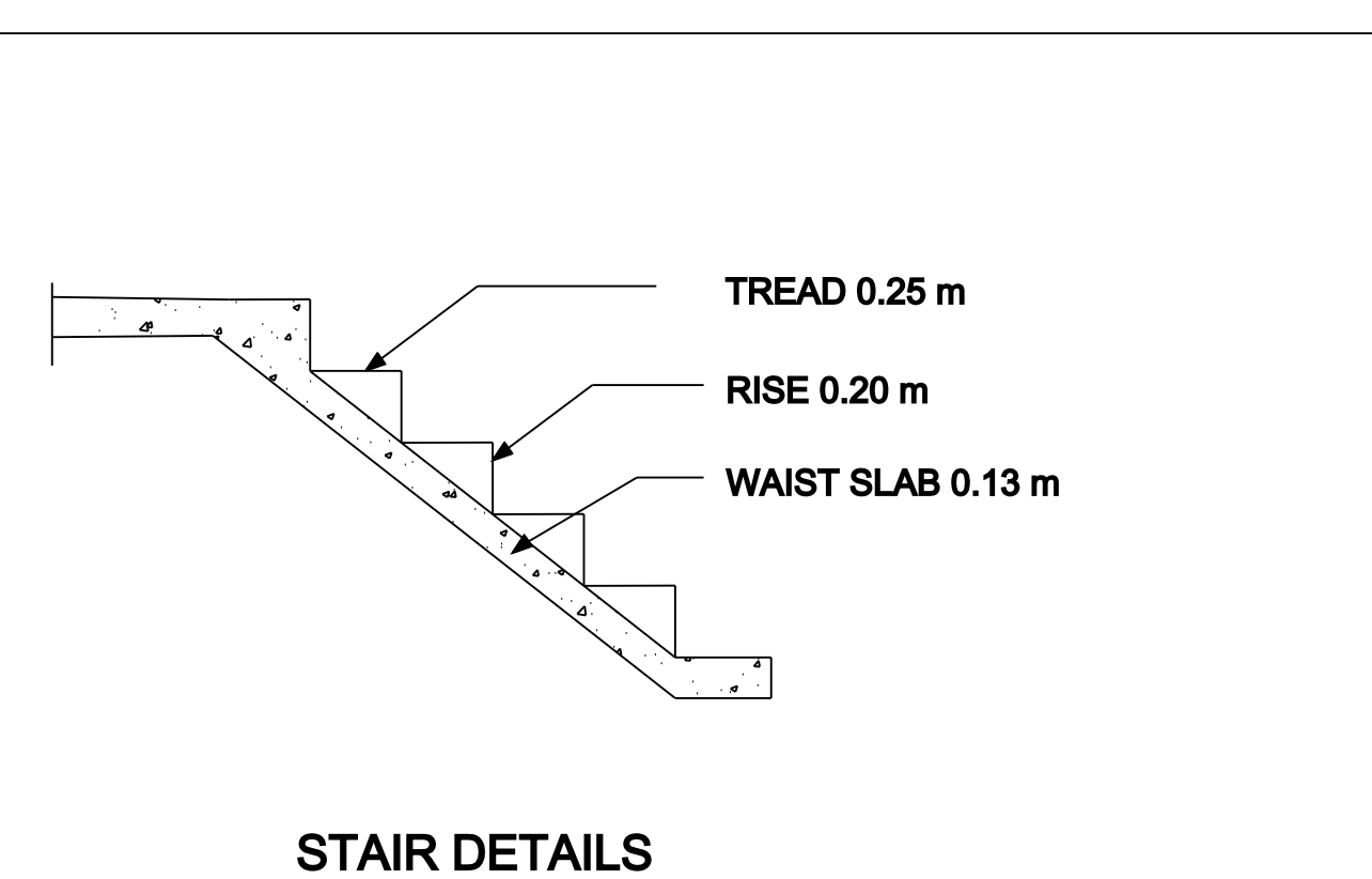
STAIR DETAILS
