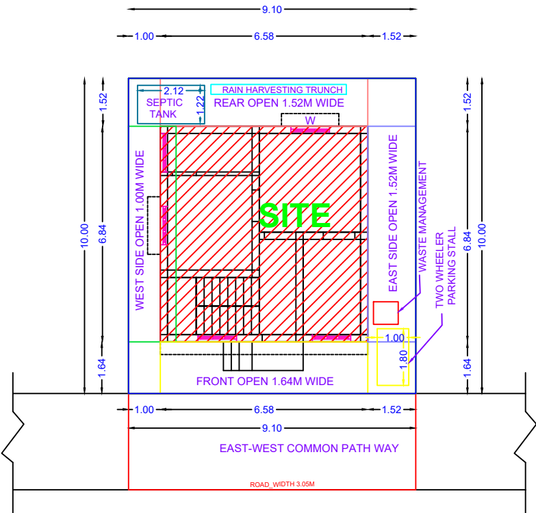
SITE PLAN
