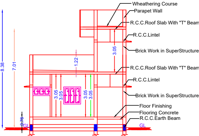
SECTION ON "PQ" SCALE 1:100
