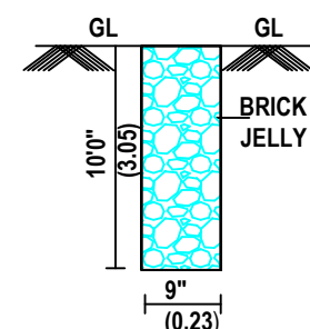
PERCULATION PIT
