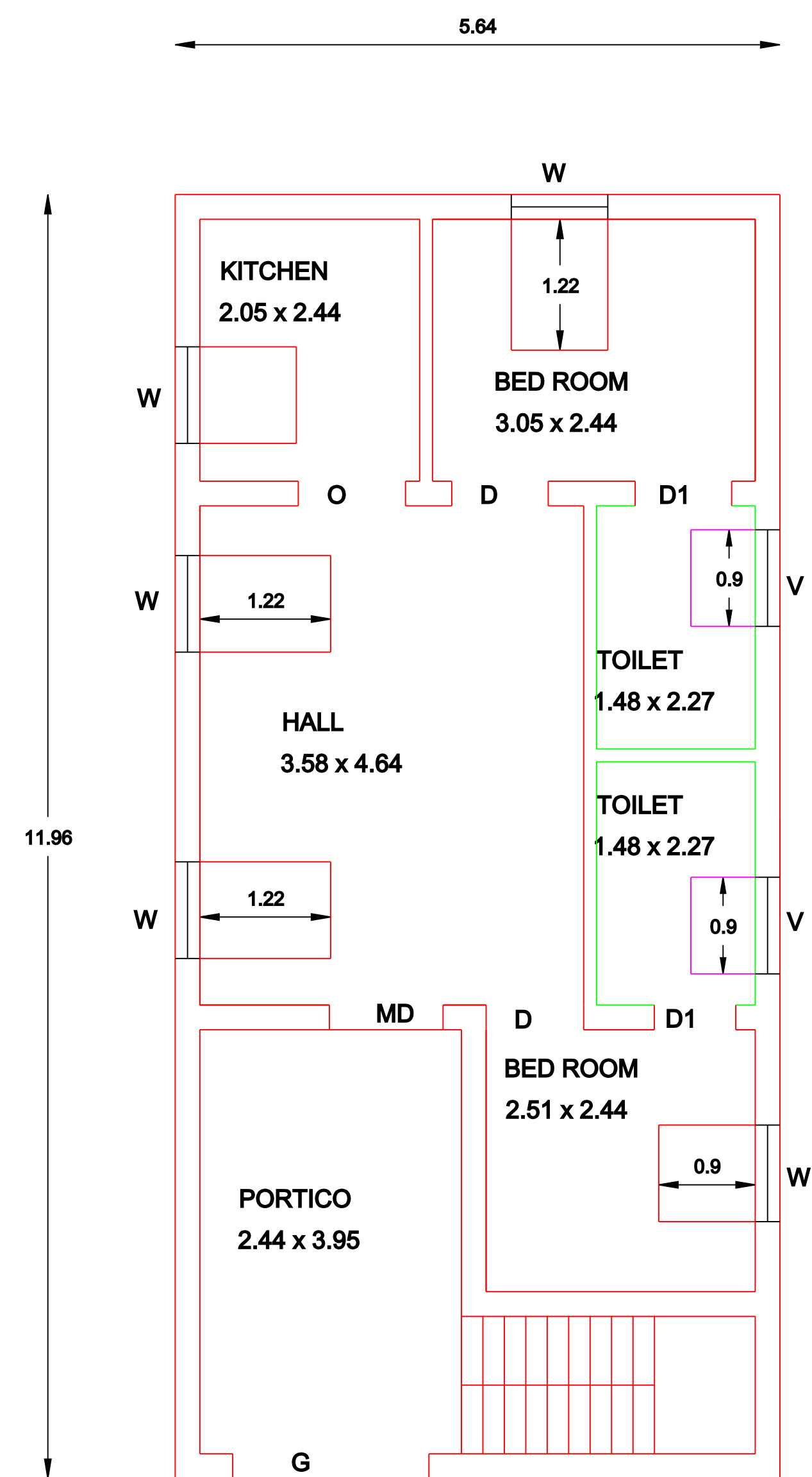
PLAN
