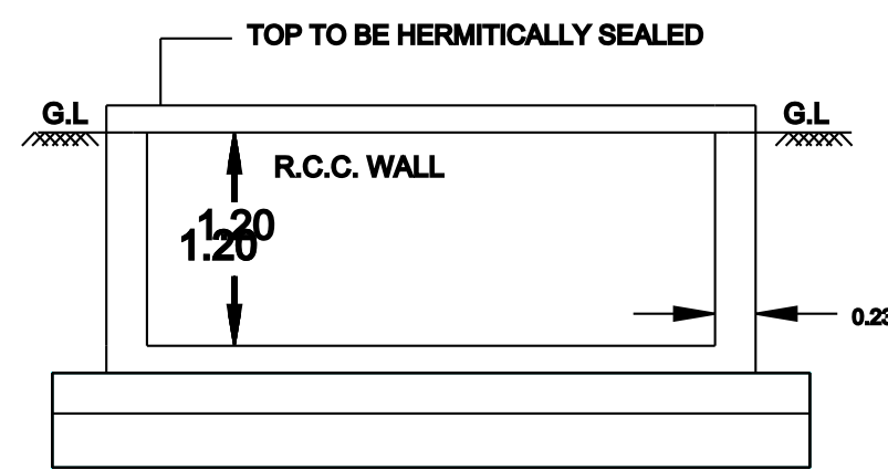
RWH SECTION
