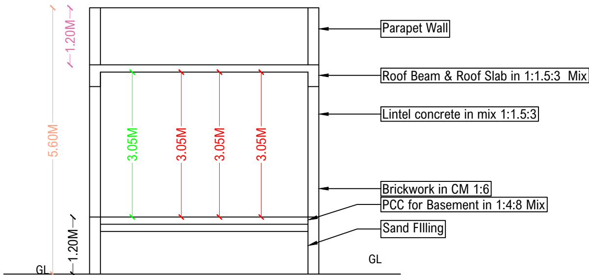
SECTION
