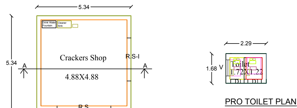
Pro. Ground Floor Plan
