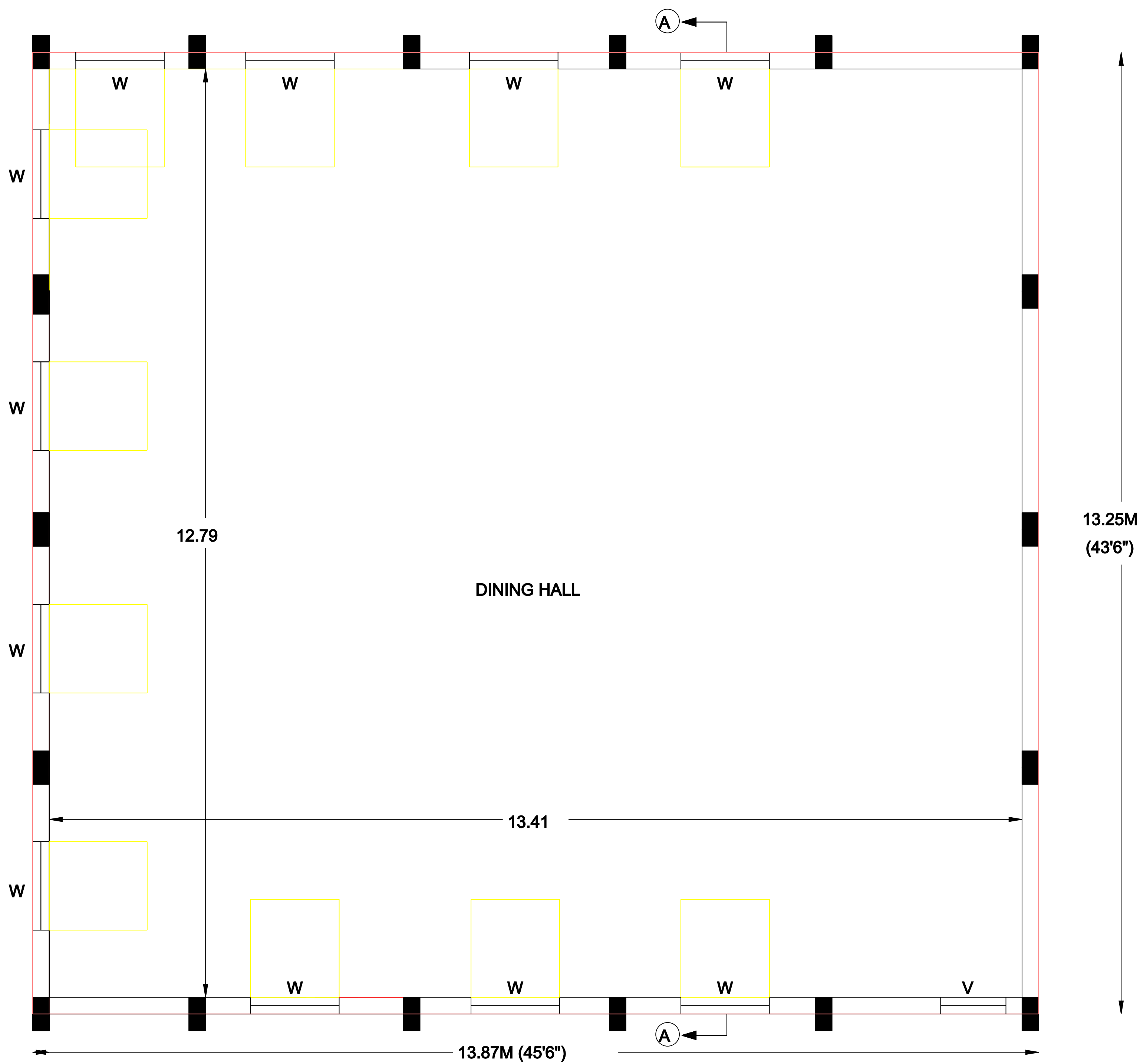
PROPOSED ADDITIONAL FIRST FLOOR PLAN
