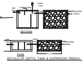
PLAN DETAILS OF SEPTIC TANK & DISPERSION TRENCH
