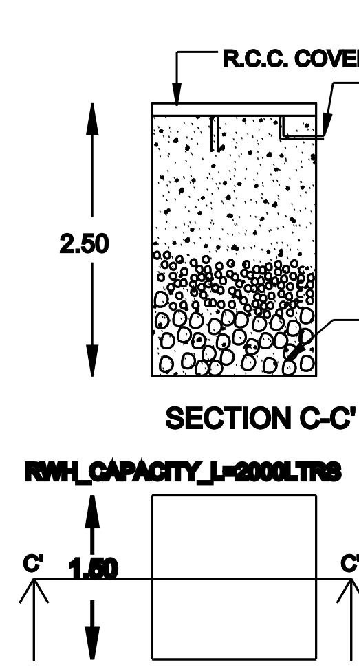
SECTION C-C'
