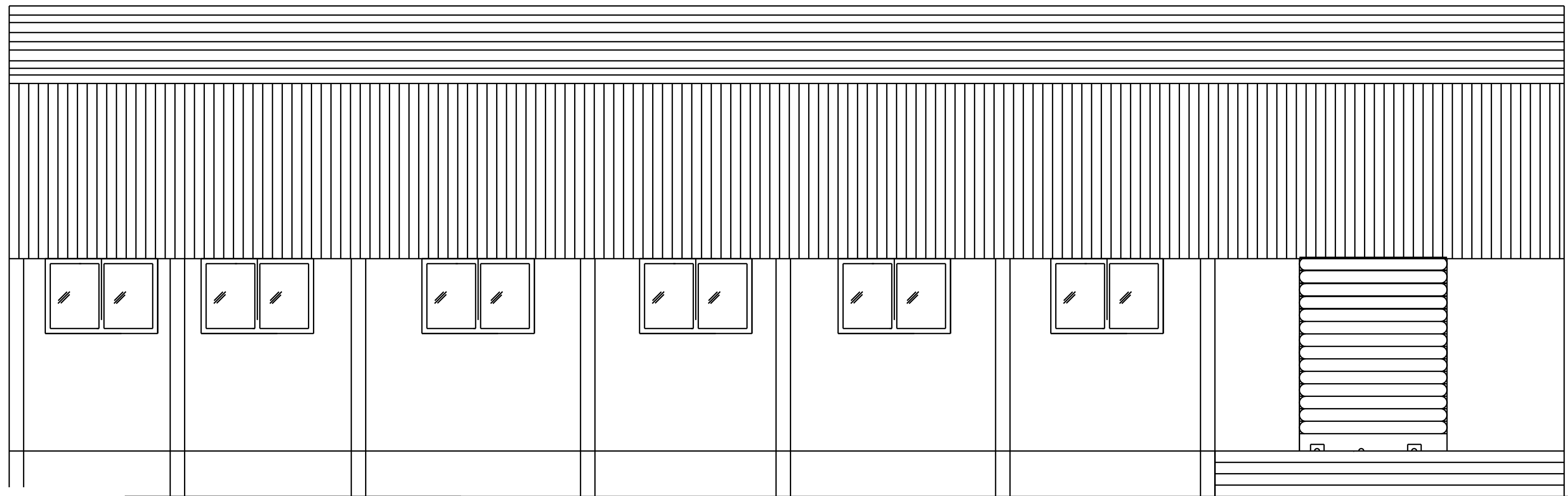
FRONT ELEVATION
