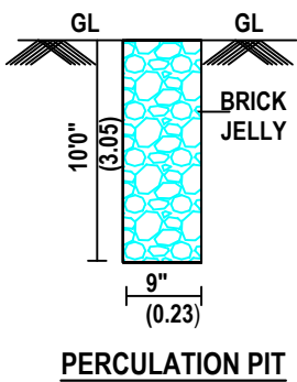
PERCULATION PIT
