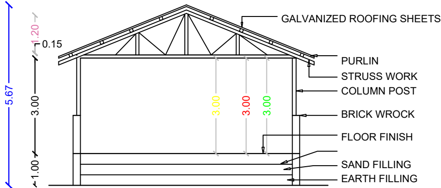
SECTION X-X
