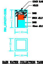
RAIN WATER COLLECTION TANK
