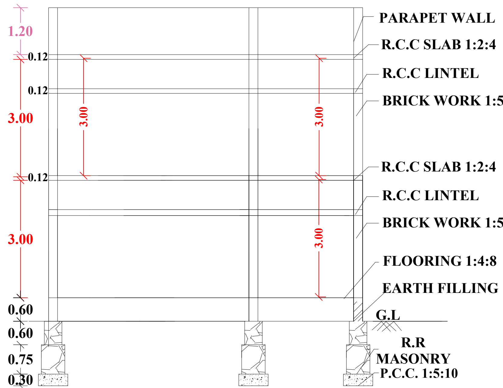
"SECTION "AB"
