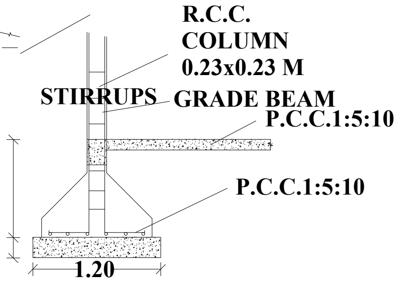
COLUMN DETAIL
