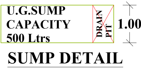
SUMP DETAIL
