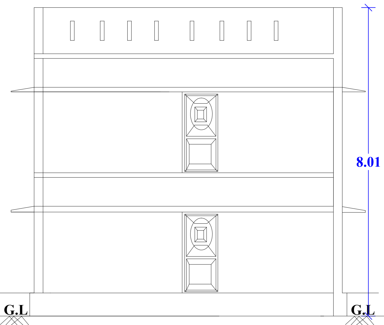
FRONT ELEVATION
