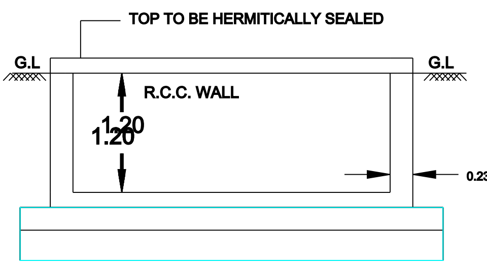
RWH SECTION
