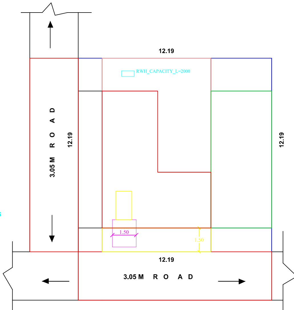
SITE PLAN
