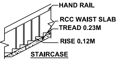
STAIRCASE
