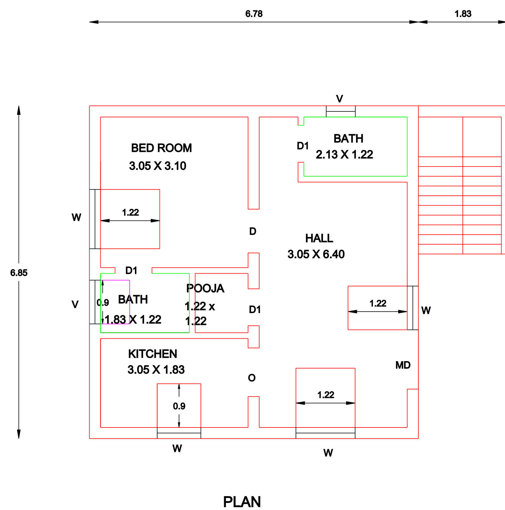
PLAN
