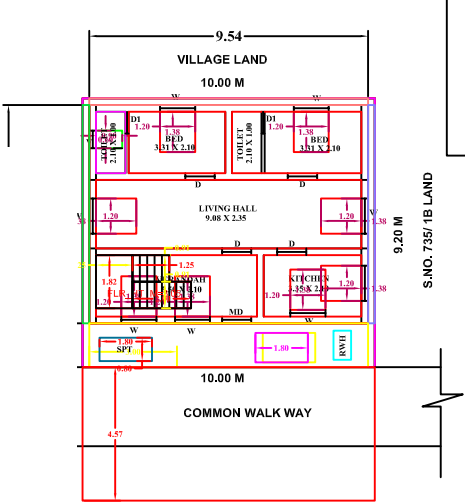
TE & GROUND FLOOR PLAN
