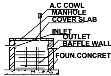
DETAILS OF SEPTIC TANK
