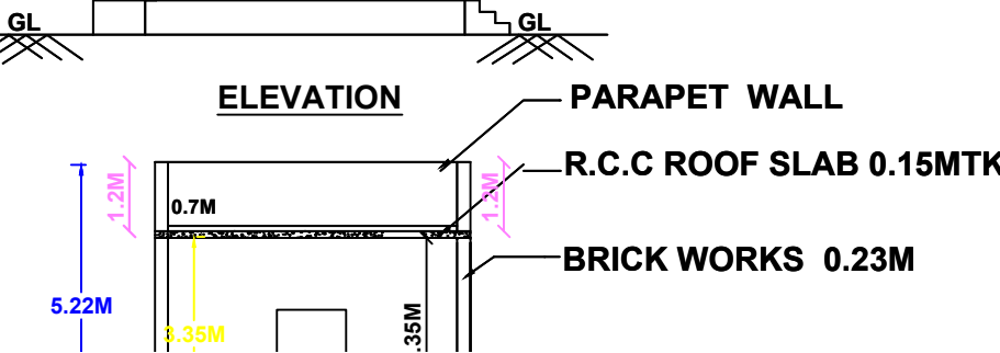
RAIN WATER HARVEST WELL
