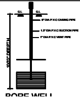
FRONT ELEVATION
