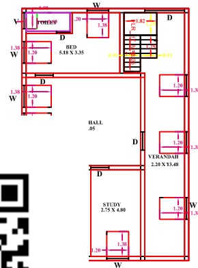
FLOOR PLAN
