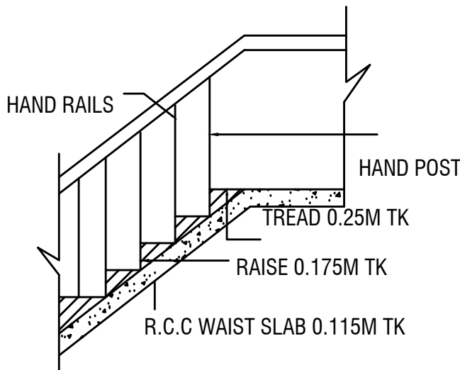
STAIRCASE DETAILS
