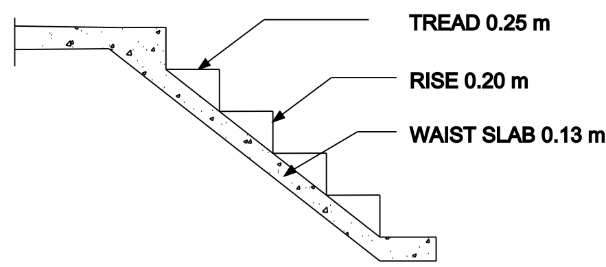
STAIR DETAILS
