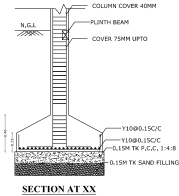
SECTION AT XX
