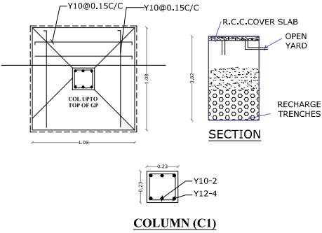
COLUMN (C1)
