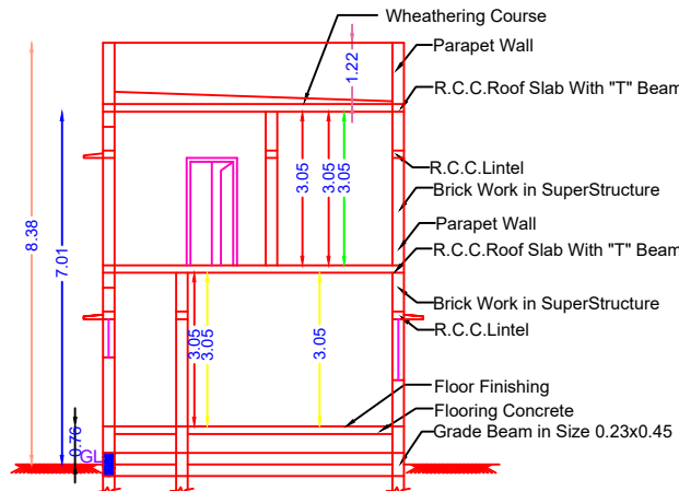
SECTION ON "PQ" SCALE 1:100
