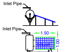
DETAILS OF SOLAR WATER HEATER
