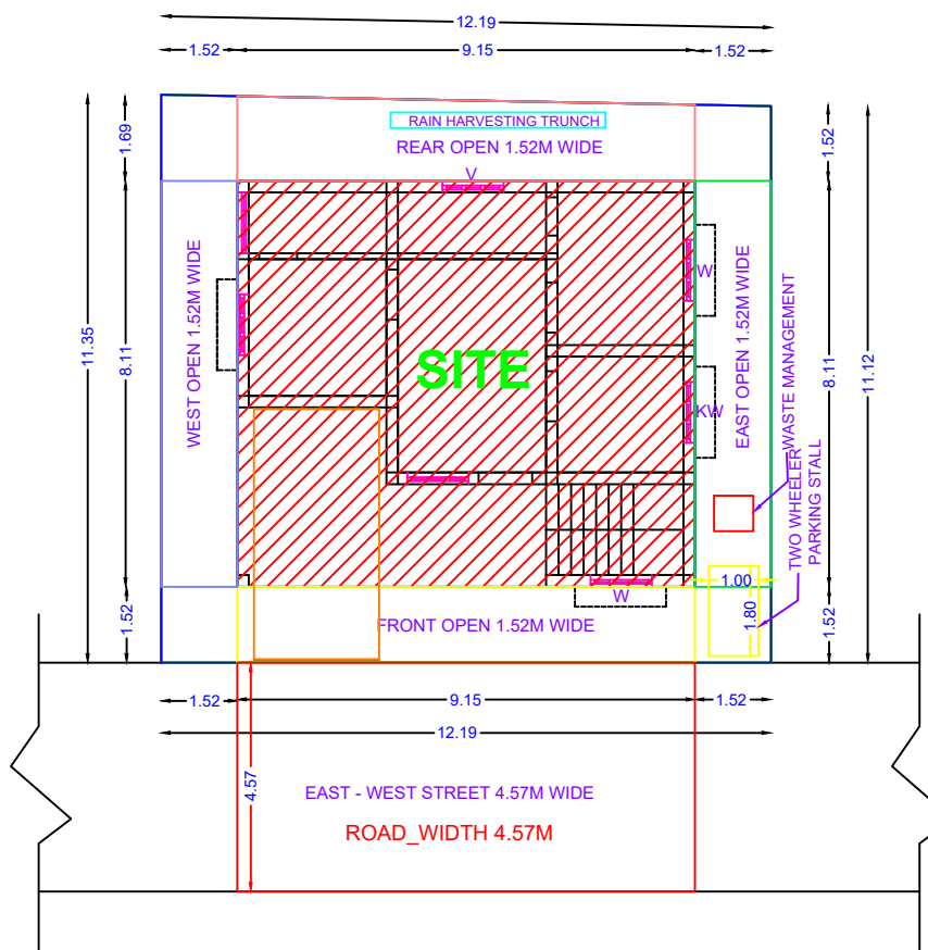
SITE PLAN
