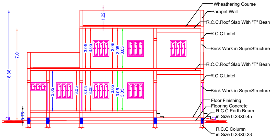
SECTION ON "PQ" (SCALE 1:100)
