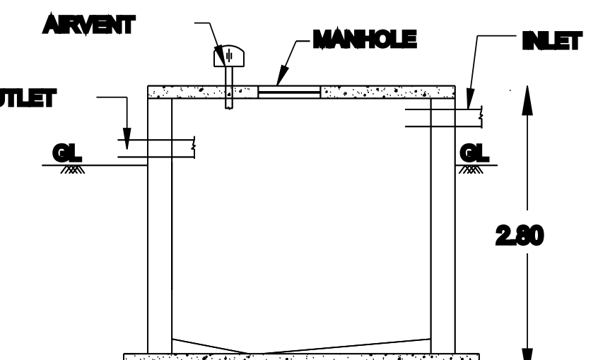
SECTION B-B'
