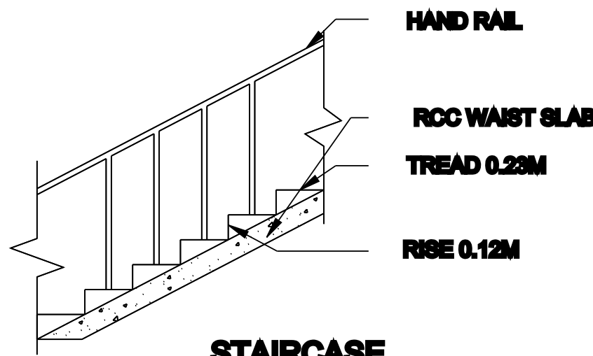
STAIRCASE
