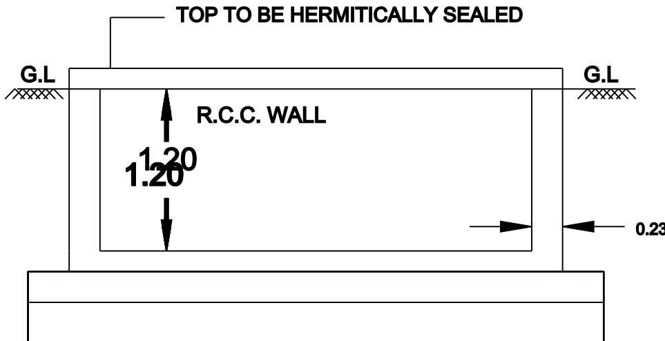
RWH_CAPACITY_L = 2000
