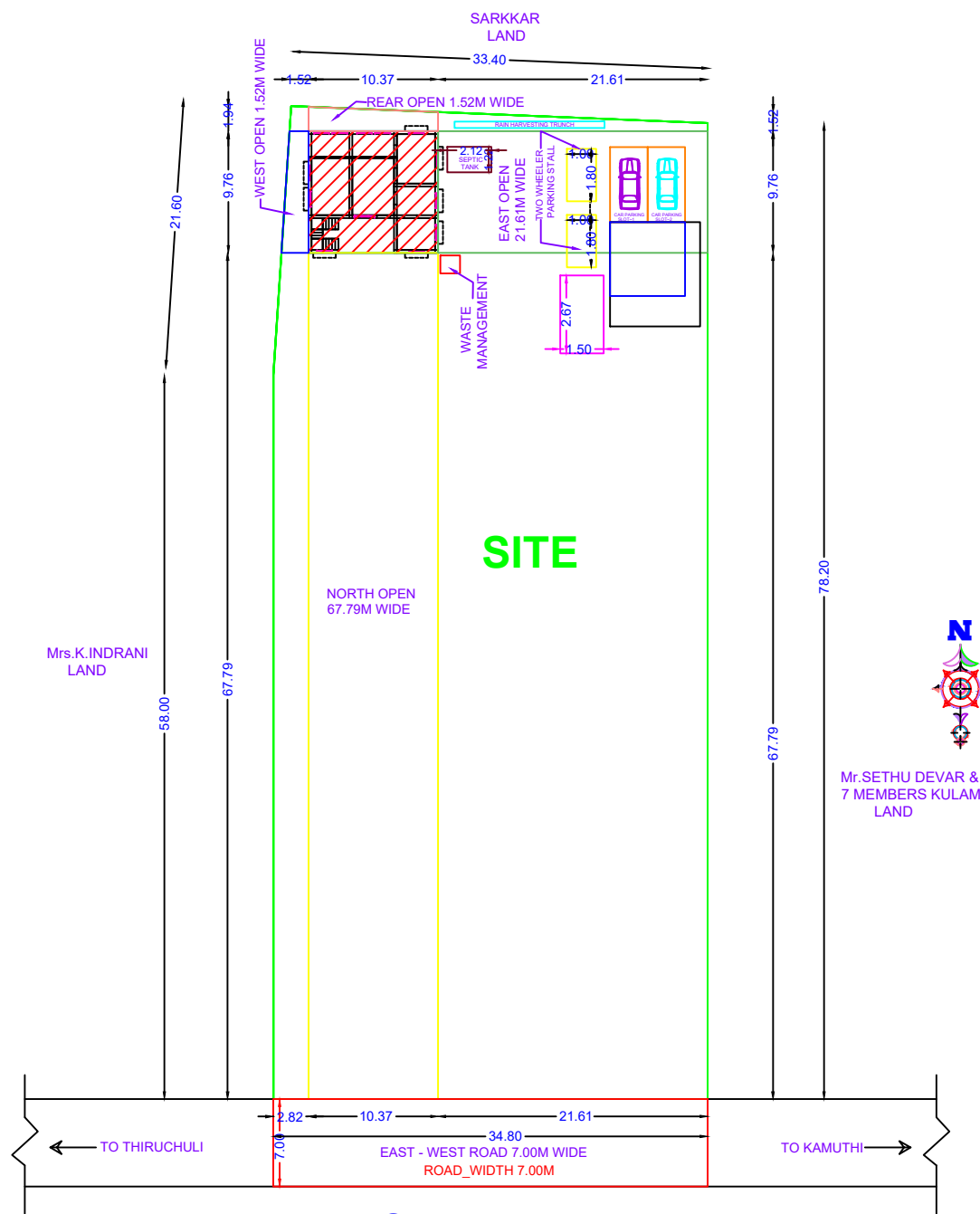
SITE PLAN
