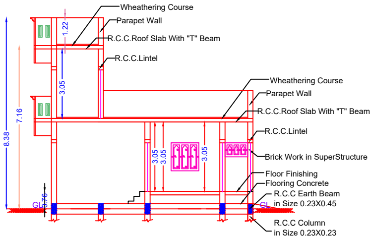
SECTION ON "PQ"
