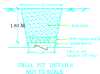
TRIAL PIT DETAILS NOT TO SCALE
