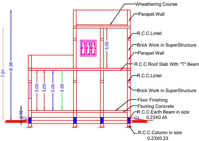
SECTION ON "PQ" SCALE 1:100
