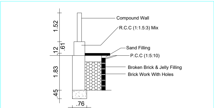
RAIN WATER HARVEST DETAILS
