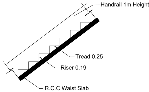
STAIR DETAILS
