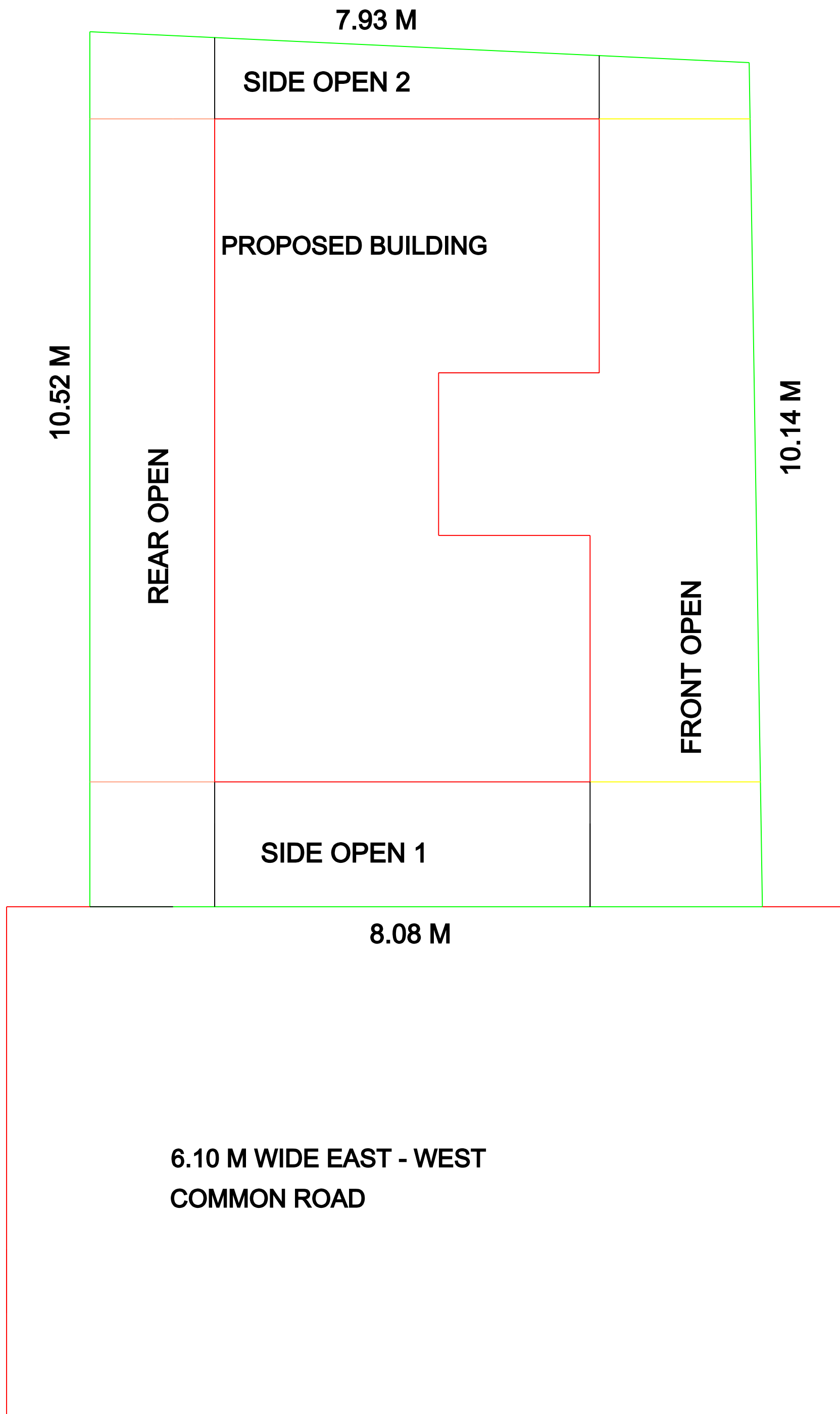
SITE PLAN
