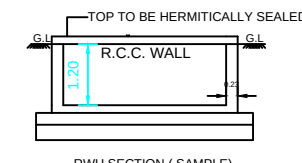
RW/1 SECTION ( SAMPLE)
