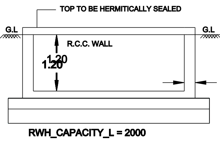
RAIN WATER HARVESTING ARRANGEMENT
