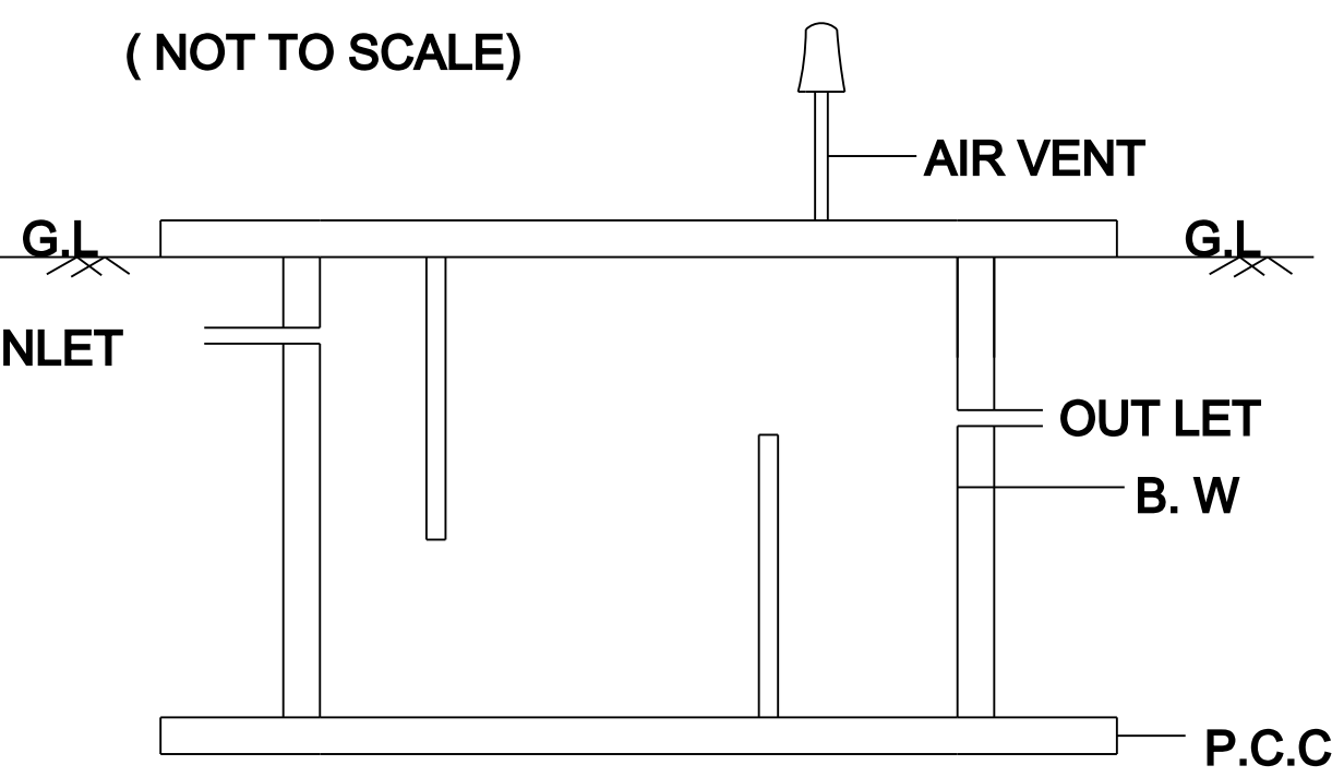
SEPTIC TANK DETAILS ( NOT TO SCALE)
