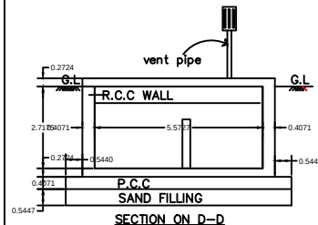
SECTION ON D-D
