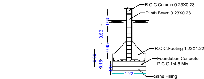
DETAILS OF COLUMN FOOTING (SCALE 1:50)
