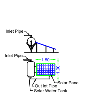
DETAILS OF SOLAR WATER HEATER
