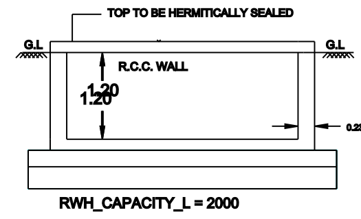
RAIN WATER HARVESTING ARRANGEMENT
