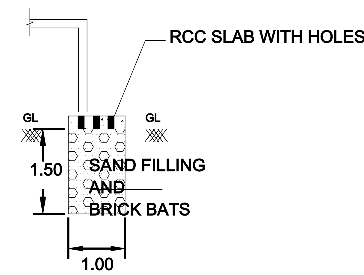
SECTION OF BS
