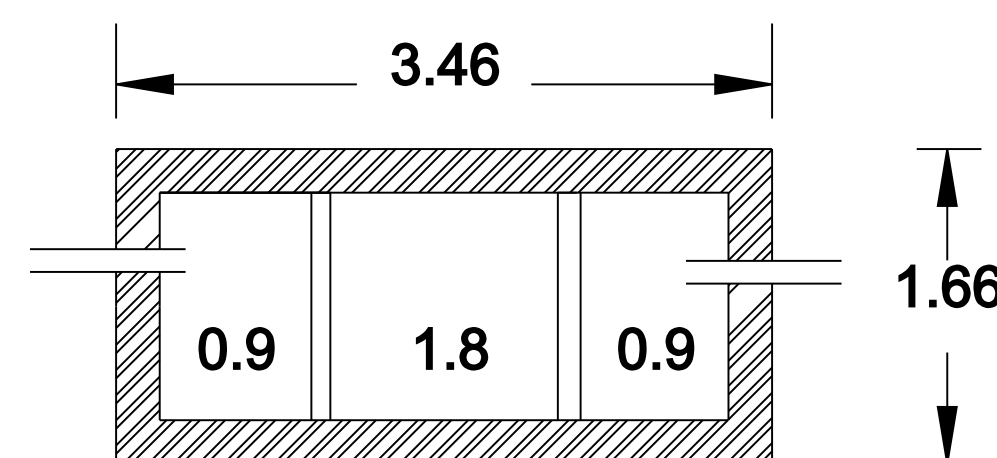
PLAN ON SEPTICTANK
