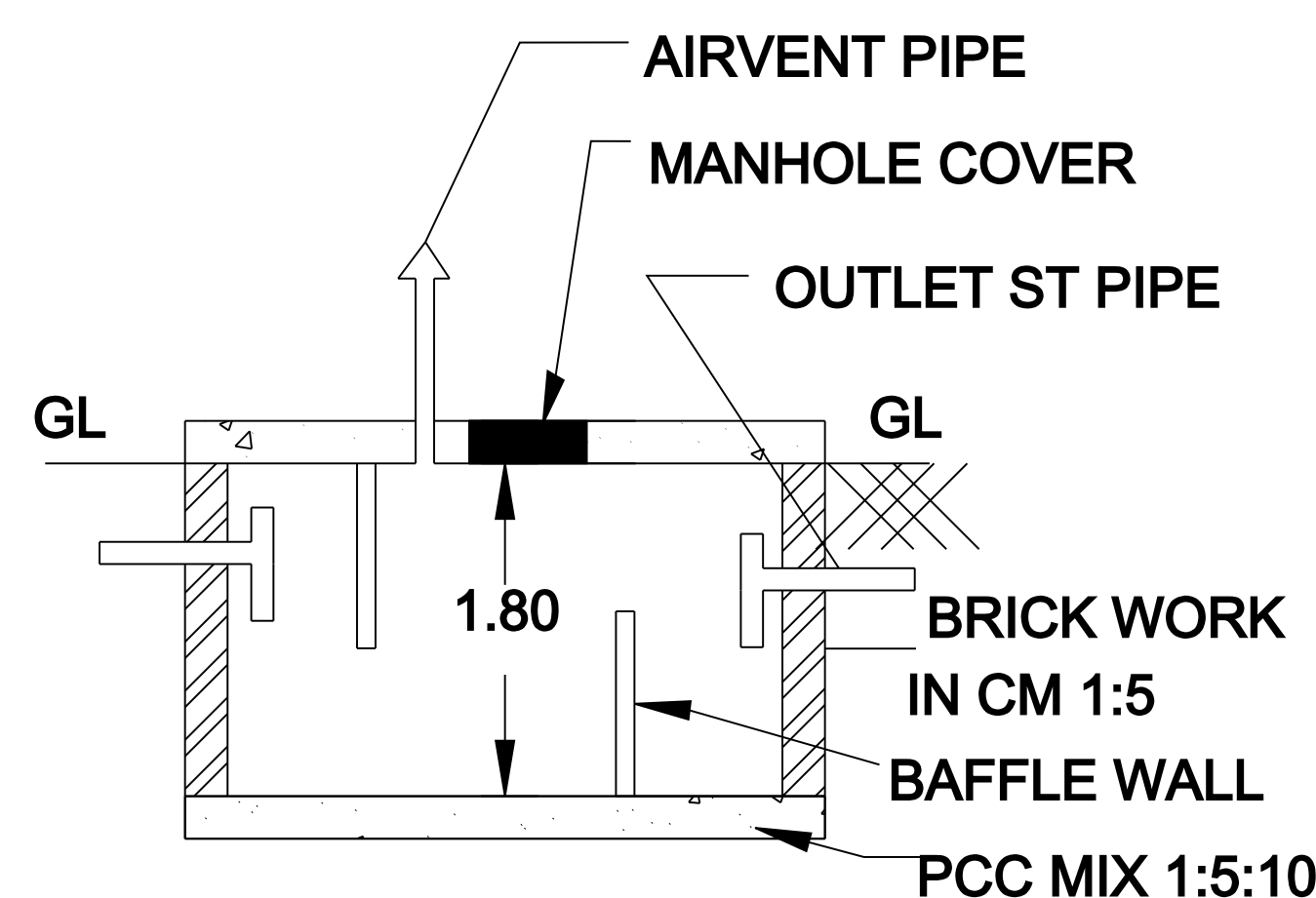
SECTION ON SEPTICTANK
