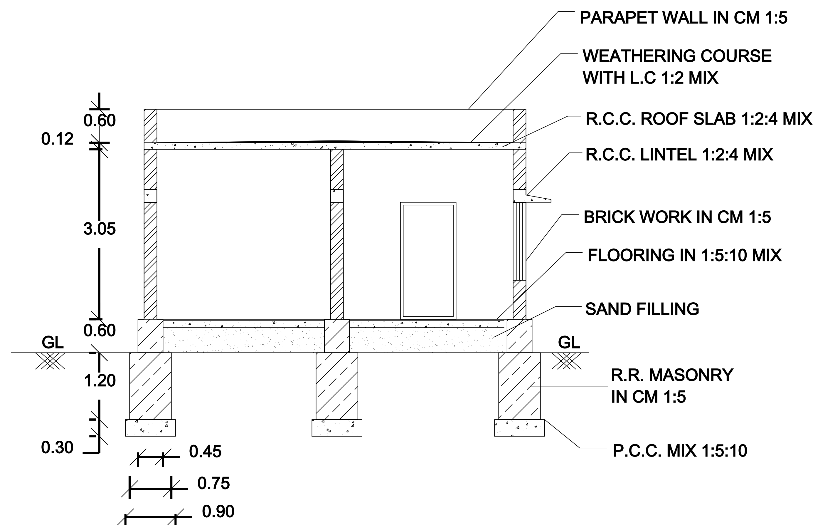
SECTION OF "AB"
