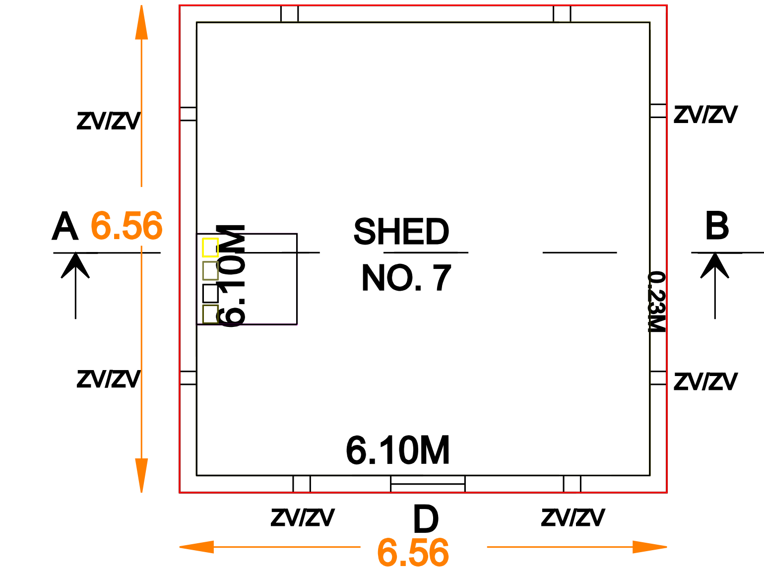
PLAN FOR SHED NO. 7
