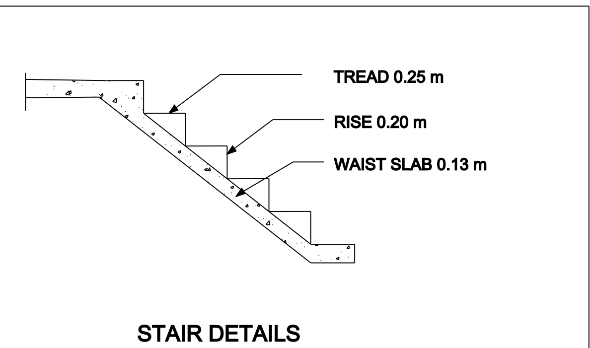
STAIR DETAILS
