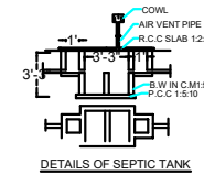
DETAILS OF SEPTIC TANK
