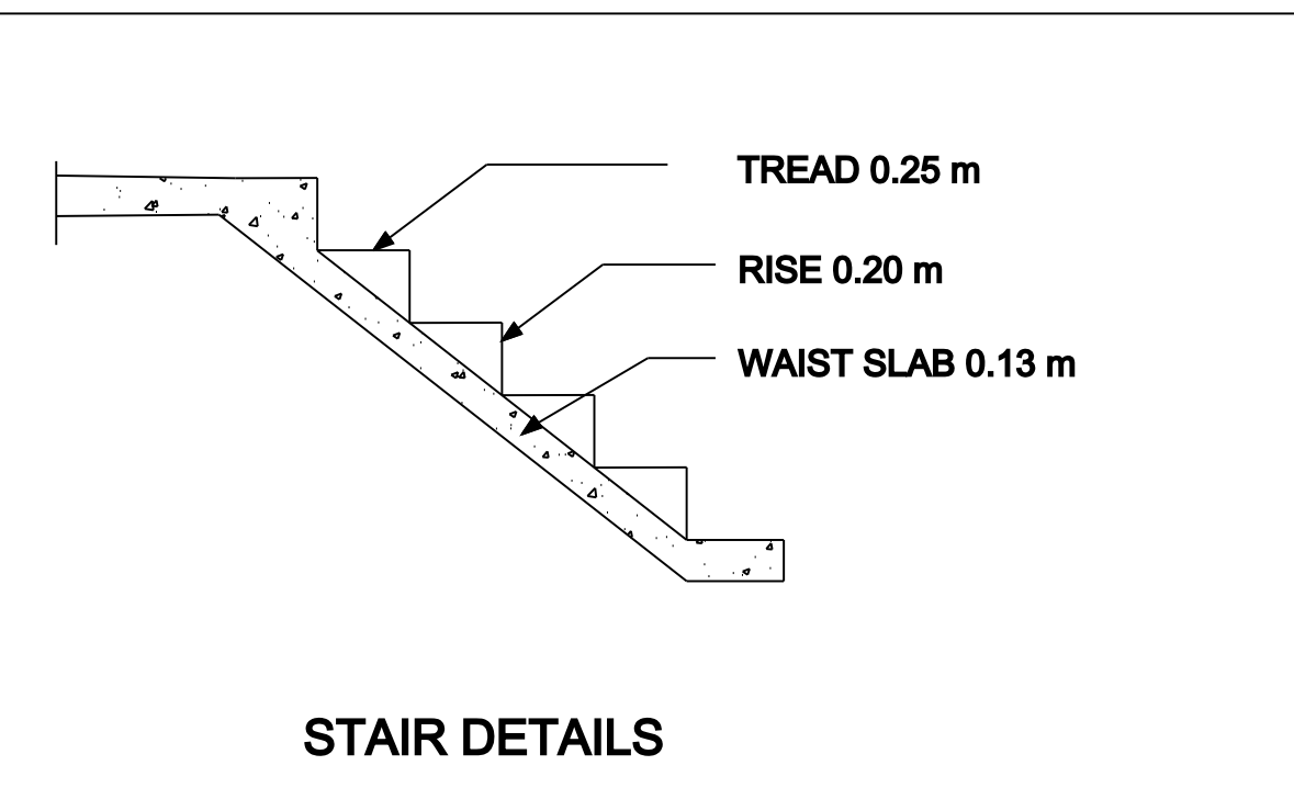
STAIR DETAILS
