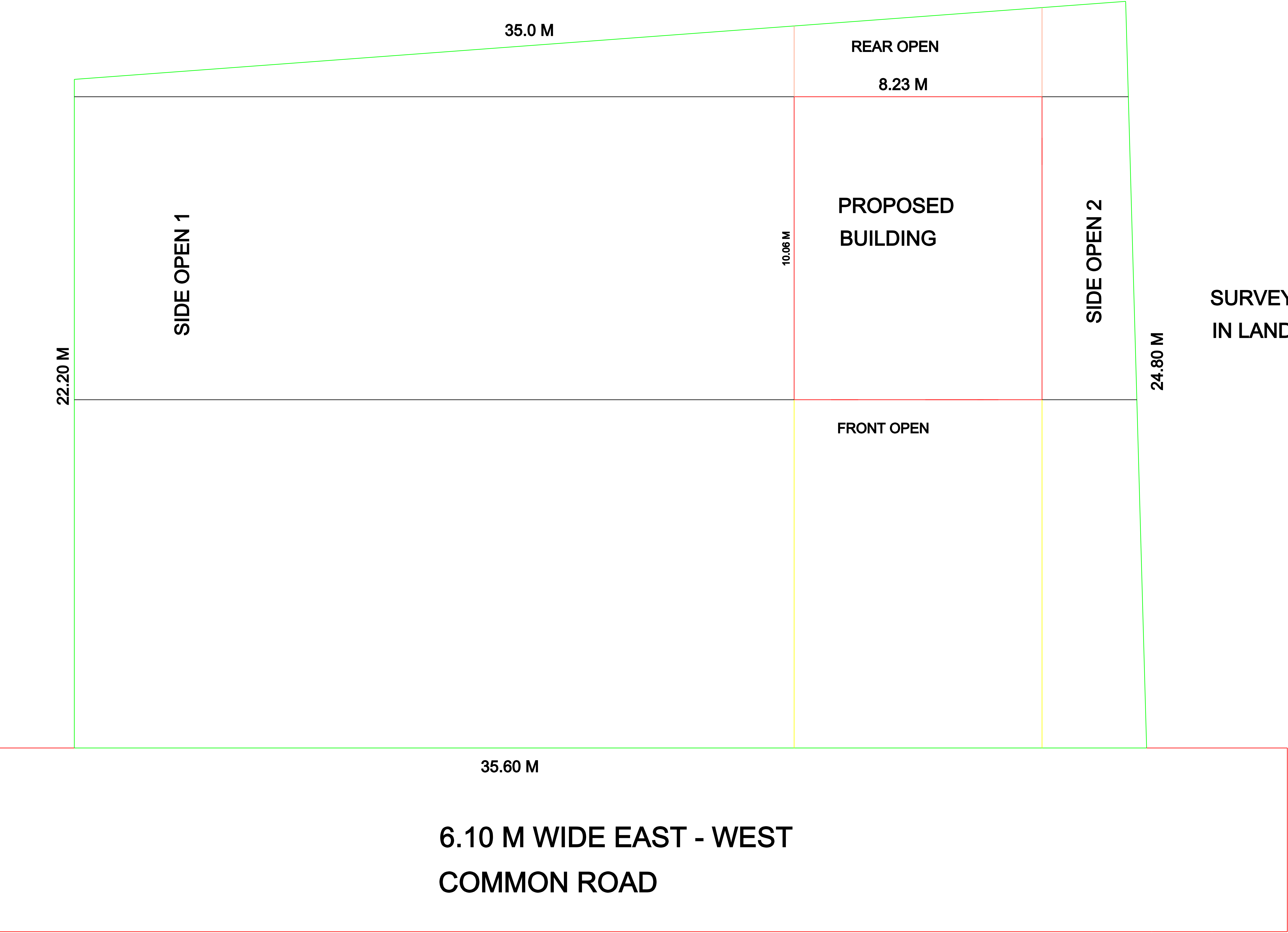
SITE PLAN
