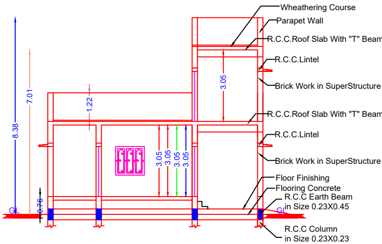
SECTION ON "PQ" (SCALE 1:100)
